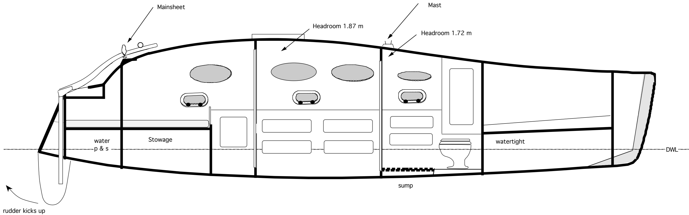
Port Hull Centreline section
