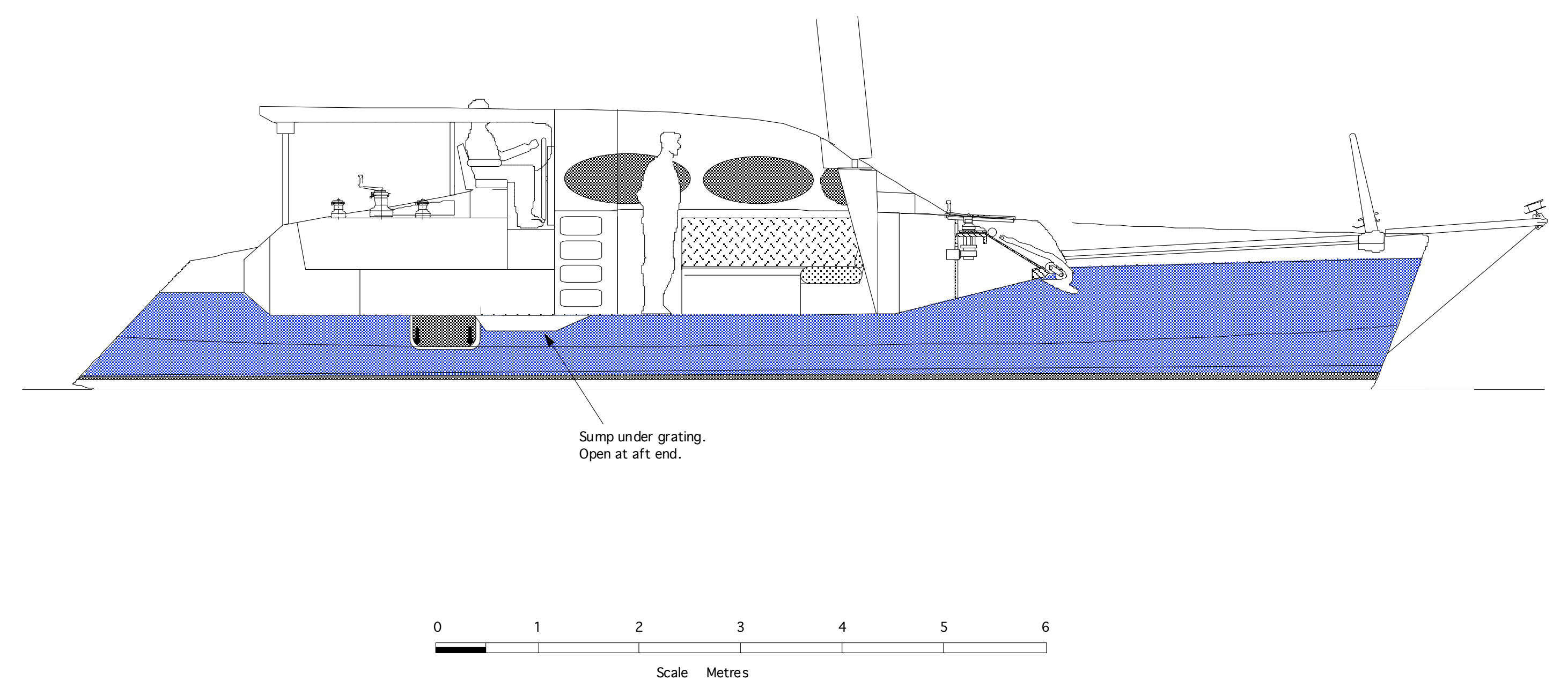
John Shuttleworth Yacht Designs Ltd. © 2005. Centrelines section FOR Boiling Frog Scale 1:40 Study 1 Cerys (Advantage 44 Mk 3)
