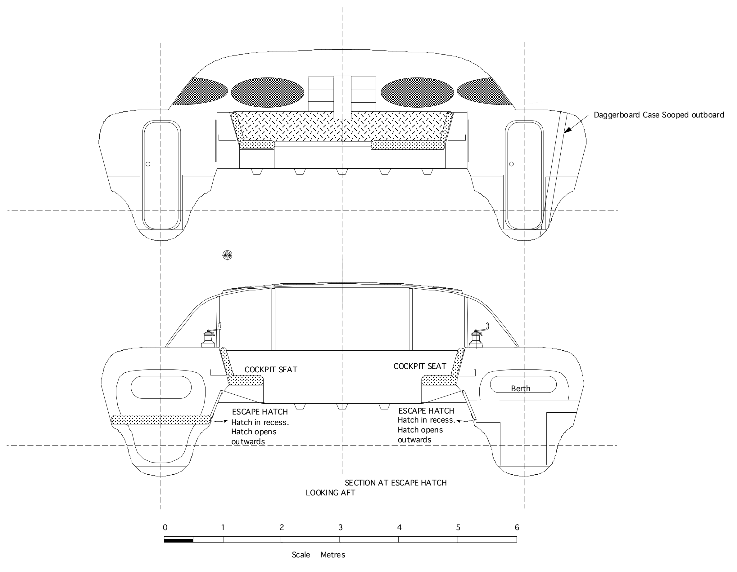
John Shuttleworth Yacht Designs Ltd. © 2005. Hull Sections FOR Boiling Frog Scale 1:40 Study 1 Cerys (Advantage 44 Mk 3)
