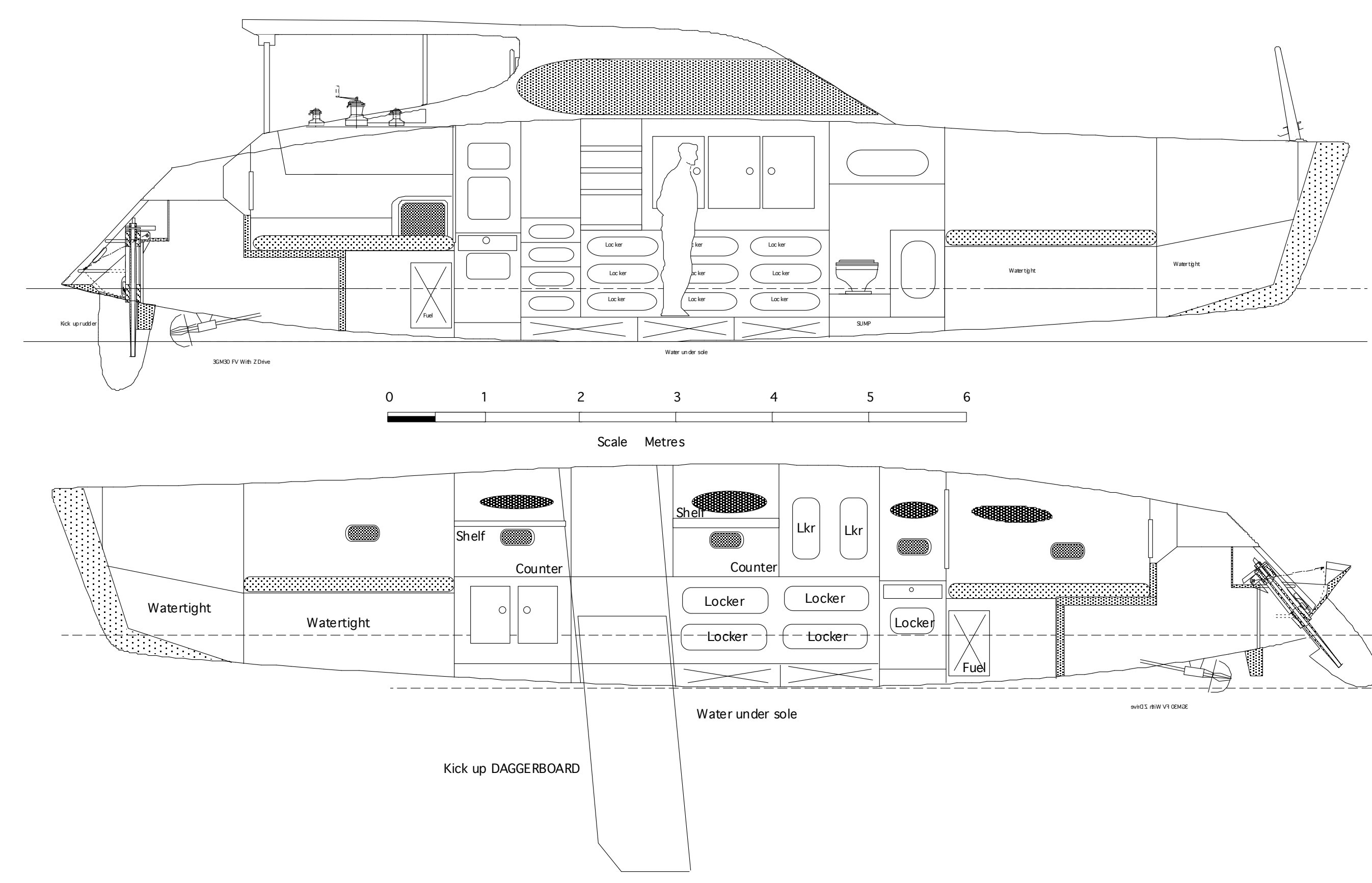
John Shuttleworth Yacht Designs Ltd. © 2005. Hull Profile Sections FOR Boiling Frog Scale 1:40 Study 1 Cerys (Advantage 44 Mk 3)
